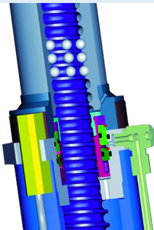
SST stands for SAFETY STAR TECHNOLOGY, a patented NUSSBAUM-technology regulating and monitoring the synchronization of both lift columns to 1/16"
