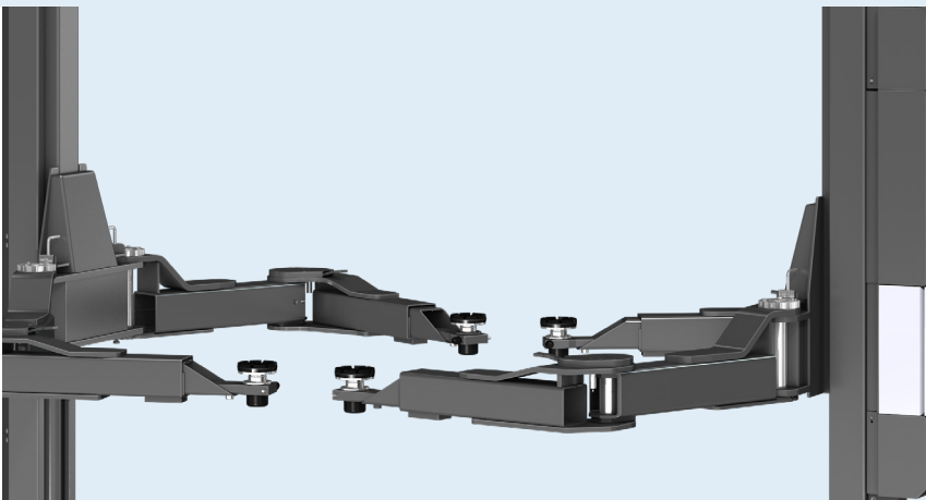
OTTO arms: flexible and user friendly, reaching 100% of pick-up points. Pneumatic arm restraints standard on the HDL 18
