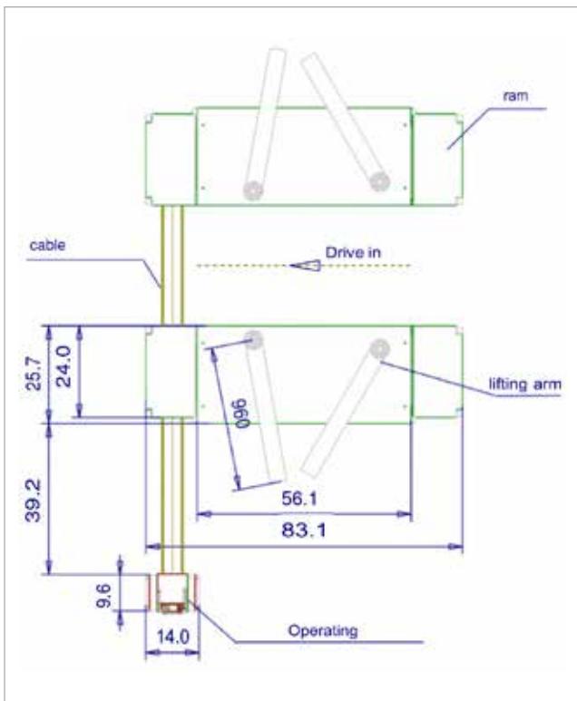
Quick Lube NT Technical Drawings
