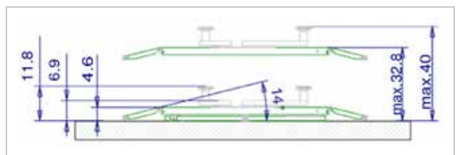
Quick Lube NT has no mechanical ties between platforms eliminating work obstructions
